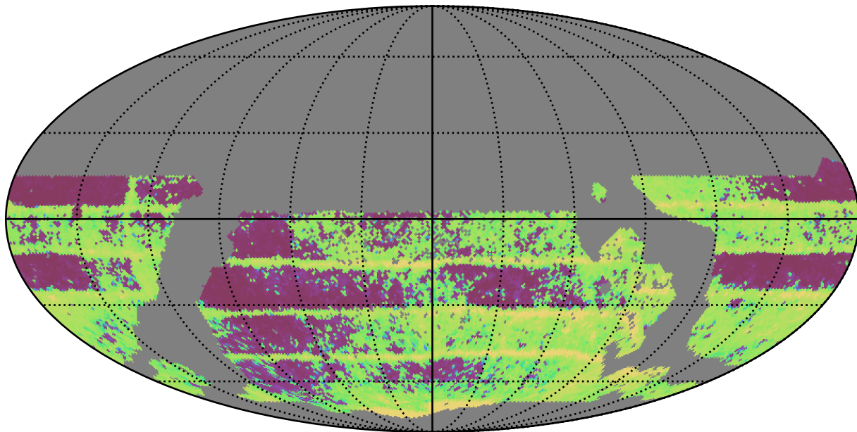
mw_roll_bulge_v3.3_10yrs WFD all bands: Median Inter-Night Gap
