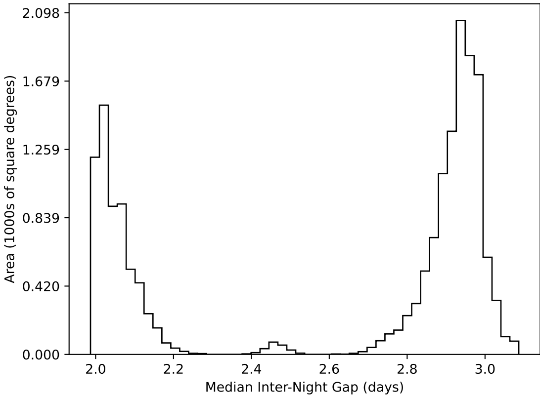
mw_roll_bulge_v3.3_10yrs WFD all bands: Median Inter-Night Gap
