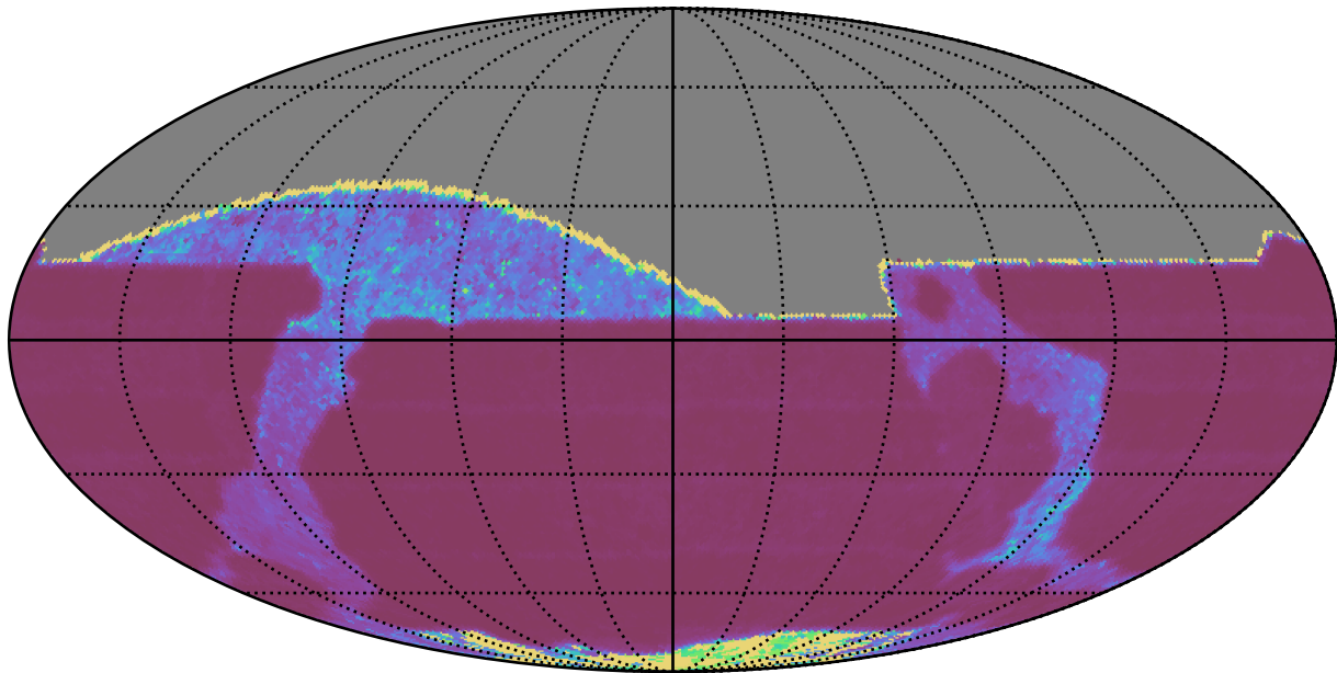
mw_roll_bulge_v3.3_10yrs All sky z band: Median Inter-Night Gap
