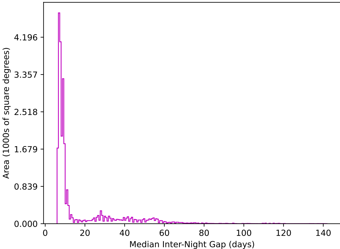
mw_roll_bulge_v3.3_10yrs All sky z band: Median Inter-Night Gap
