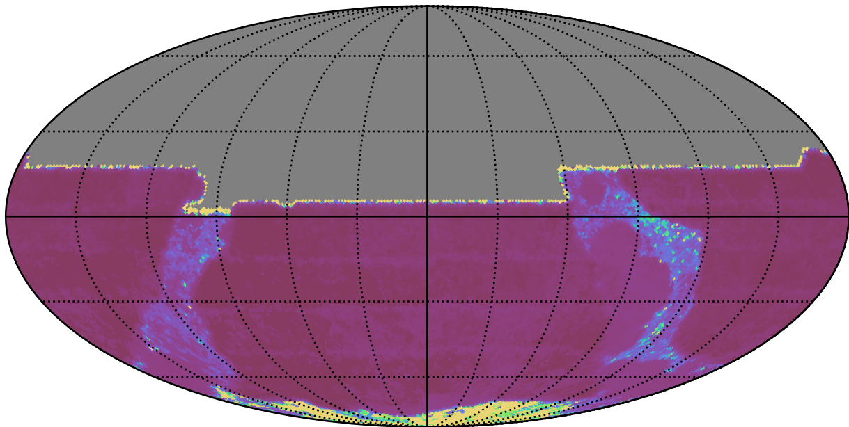
mw_roll_bulge_v3.3_10yrs All sky y band: Median Inter-Night Gap
