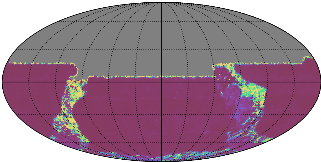
mw_roll_bulge_v3.3_10yrs All sky u band: Median Inter-Night Gap
