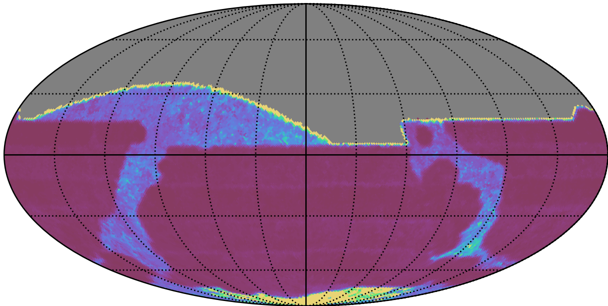
mw_roll_bulge_v3.3_10yrs All sky r band: Median Inter-Night Gap
