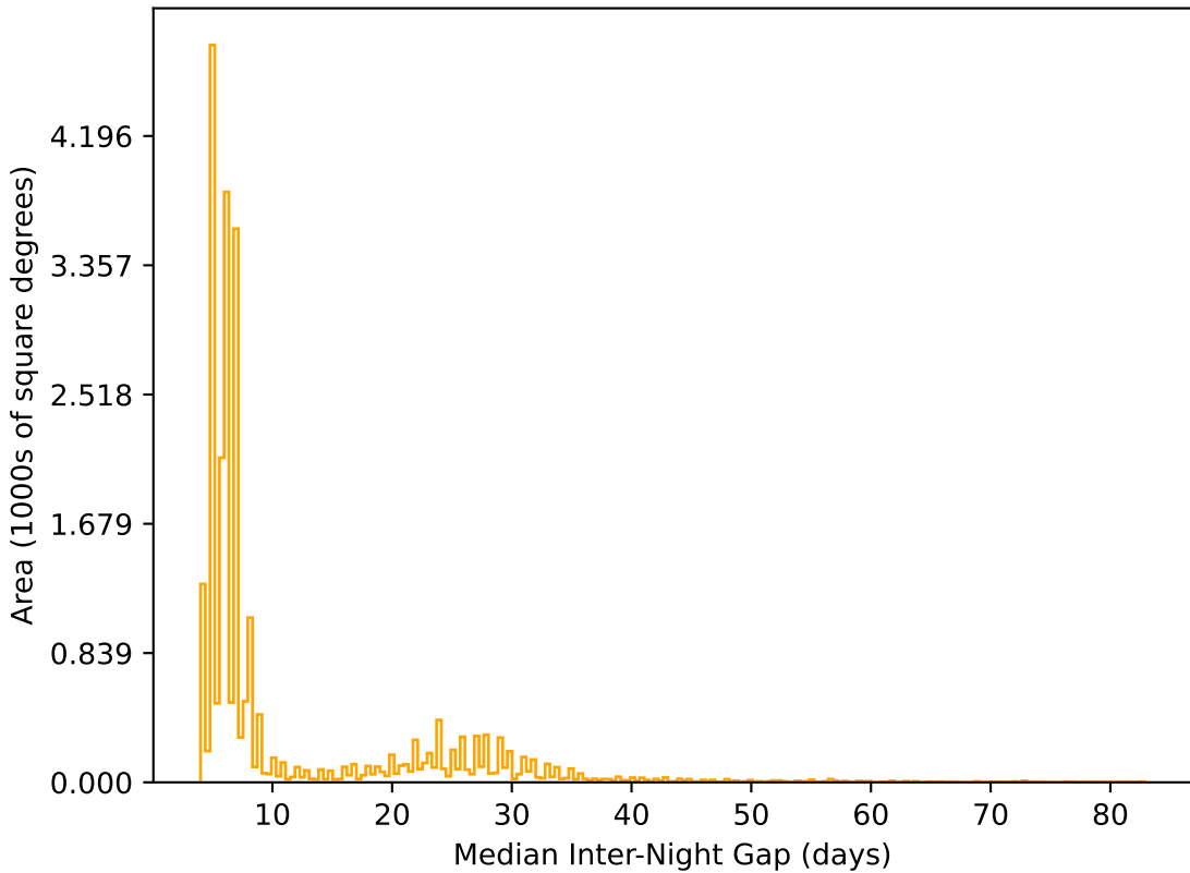
mw_roll_bulge_v3.3_10yrs All sky r band: Median Inter-Night Gap
