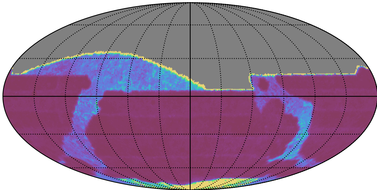
mw_roll_bulge_v3.3_10yrs All sky i band: Median Inter-Night Gap
