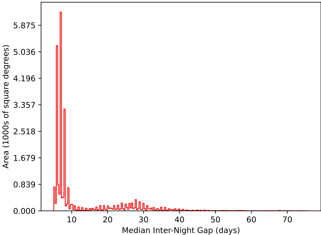
mw_roll_bulge_v3.3_10yrs All sky i band: Median Inter-Night Gap
