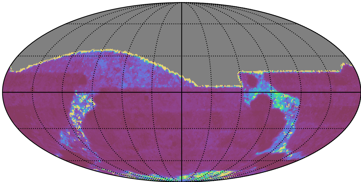
mw_roll_bulge_v3.3_10yrs All sky g band: Median Inter-Night Gap
