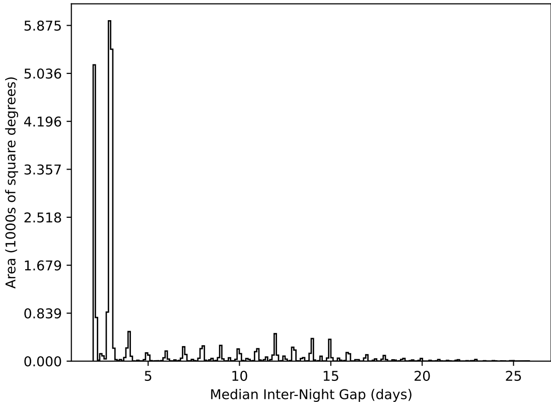
mw_roll_bulge_v3.3_10yrs All sky all bands: Median Inter-Night Gap
