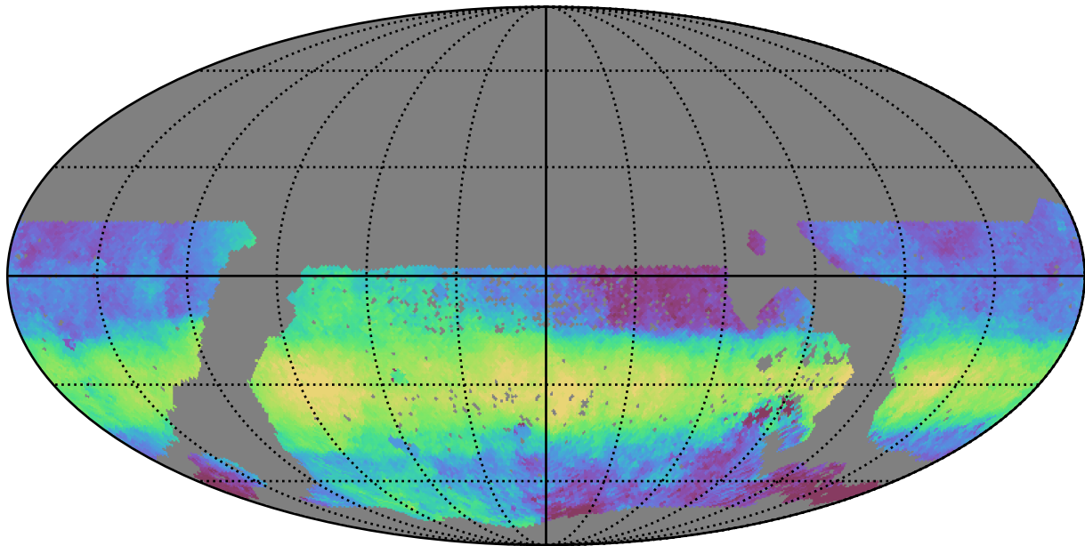
mw_roll_bulge_v3.3_10yrs WFD z band: Median HA
