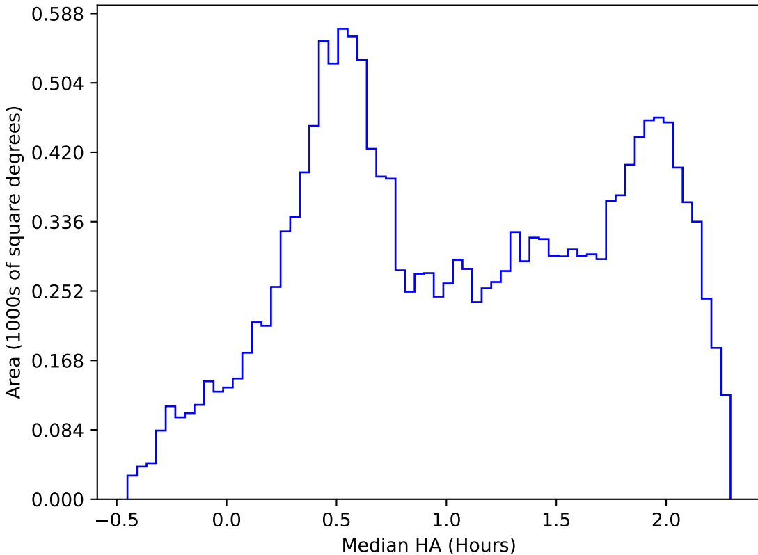
mw_roll_bulge_v3.3_10yrs WFD z band: Median HA
