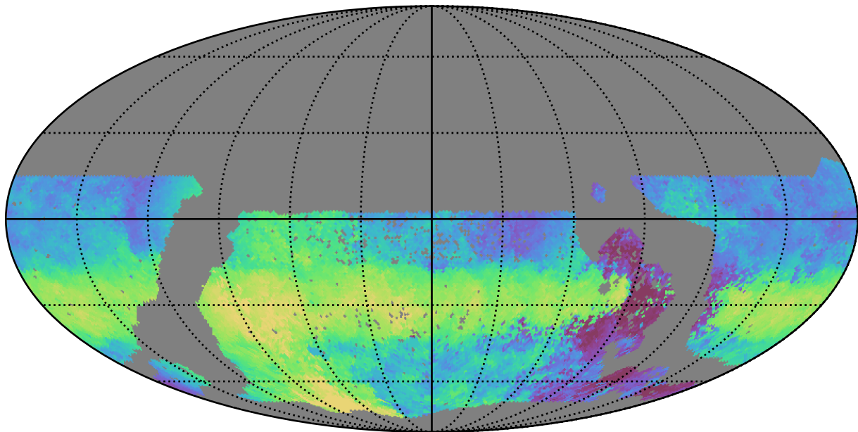
mw_roll_bulge_v3.3_10yrs WFD u band: Median HA
