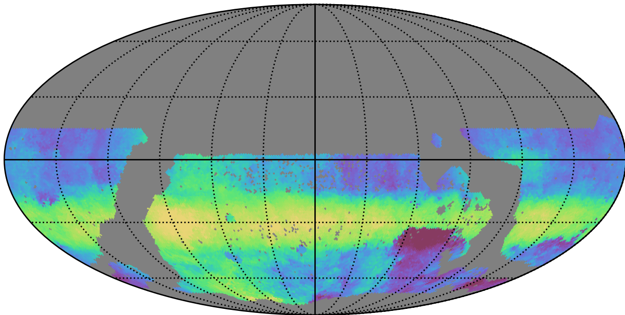
mw_roll_bulge_v3.3_10yrs WFD r band: Median HA
