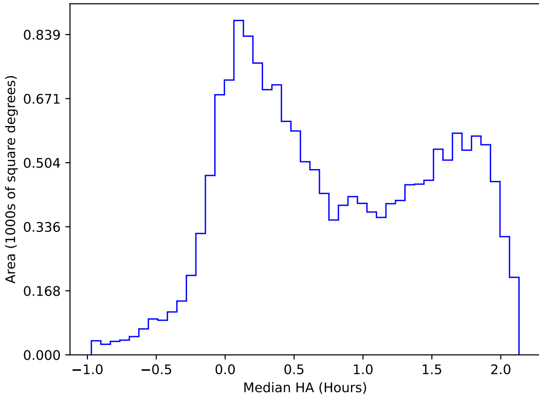
mw_roll_bulge_v3.3_10yrs WFD r band: Median HA
