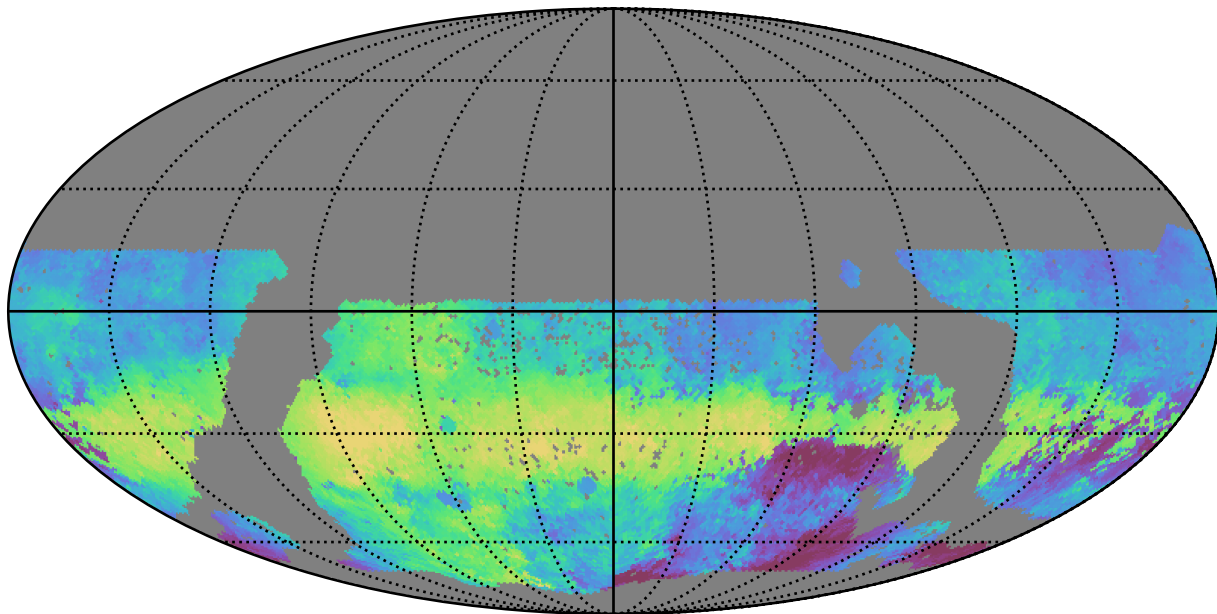
mw_roll_bulge_v3.3_10yrs WFD g band: Median HA
