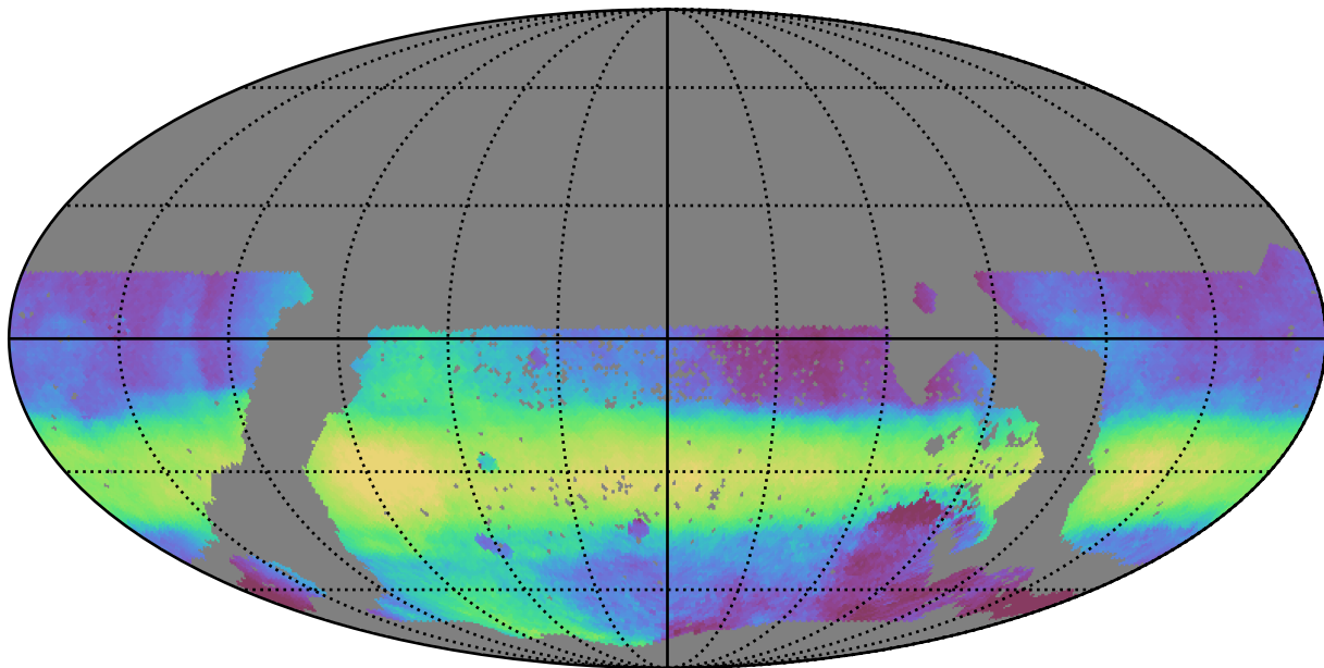
mw_roll_bulge_v3.3_10yrs WFD all bands: Median HA
