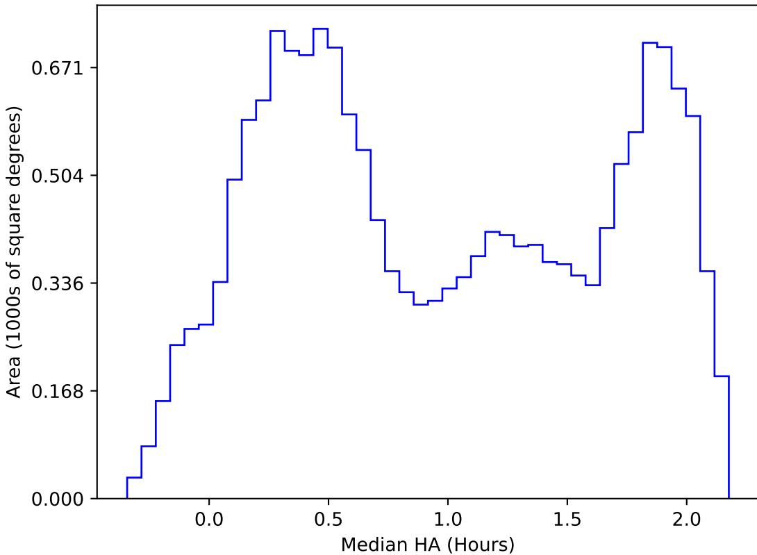
mw_roll_bulge_v3.3_10yrs WFD all bands: Median HA
