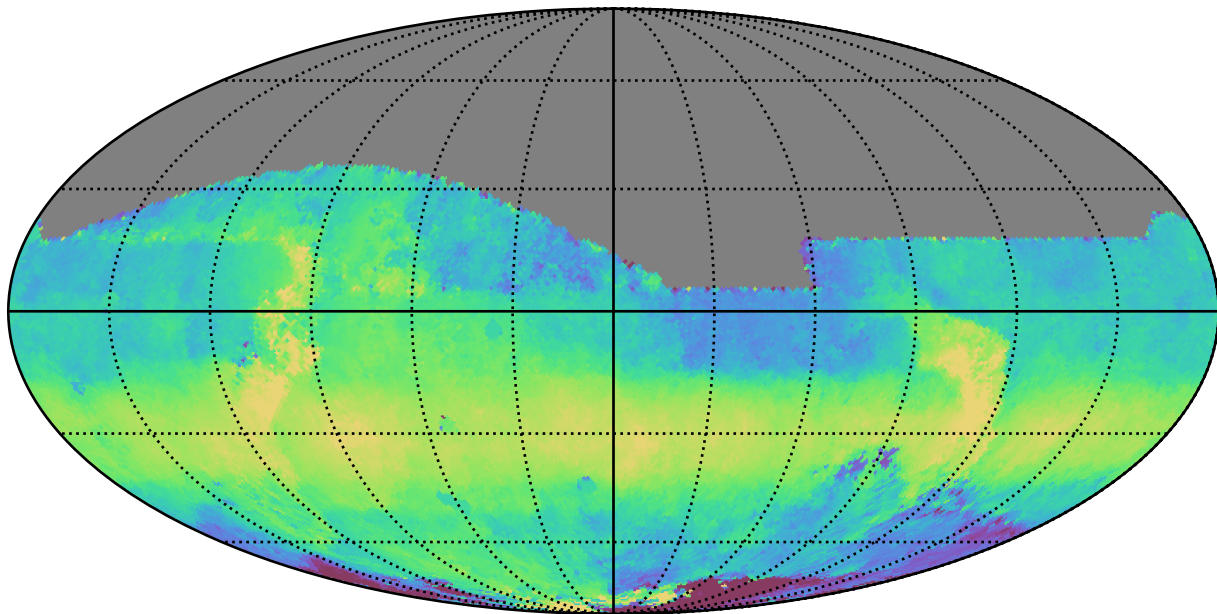
mw_roll_bulge_v3.3_10yrs All sky z band: Median HA
