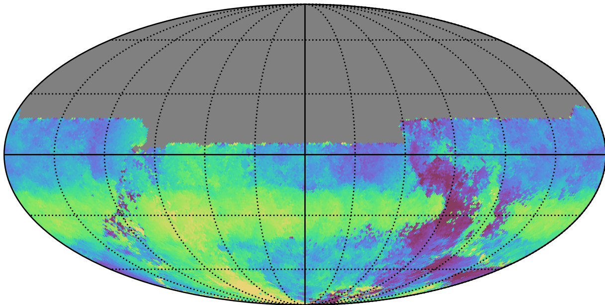
mw_roll_bulge_v3.3_10yrs All sky u band: Median HA
