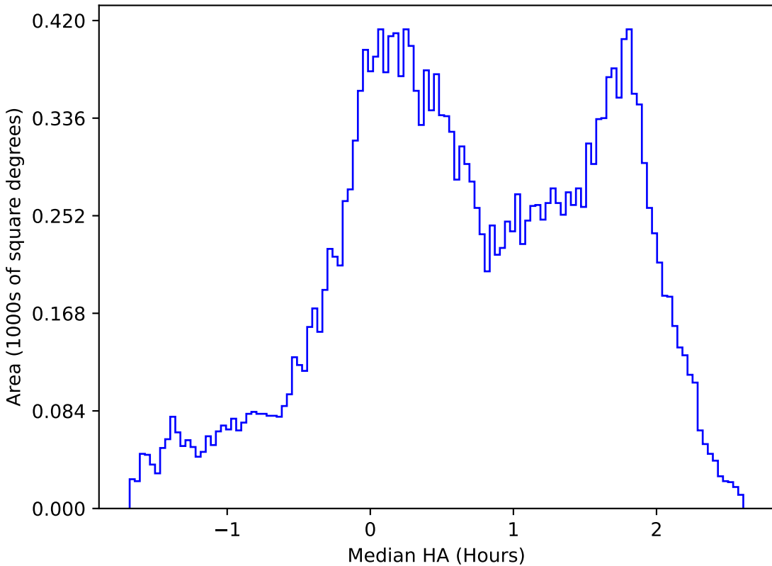
mw_roll_bulge_v3.3_10yrs All sky u band: Median HA
