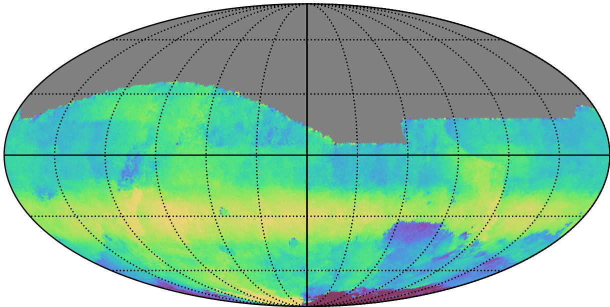
mw_roll_bulge_v3.3_10yrs All sky r band: Median HA
