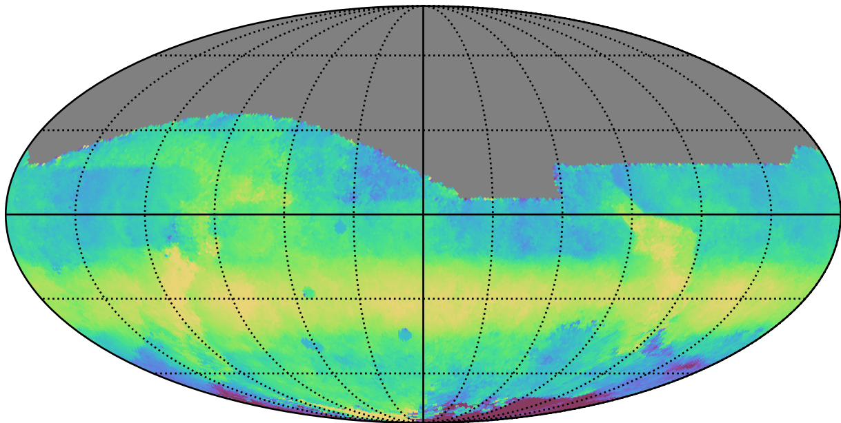
mw_roll_bulge_v3.3_10yrs All sky i band: Median HA
