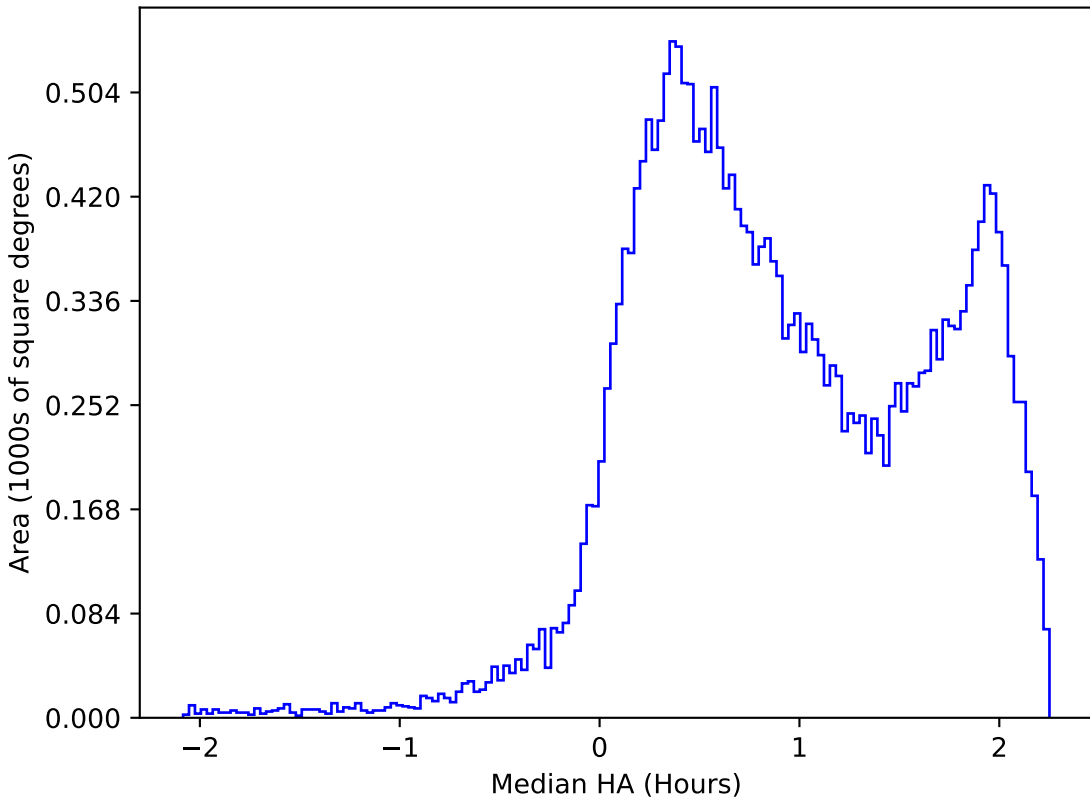
mw_roll_bulge_v3.3_10yrs All sky i band: Median HA
