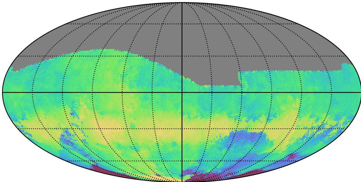
mw_roll_bulge_v3.3_10yrs All sky g band: Median HA
