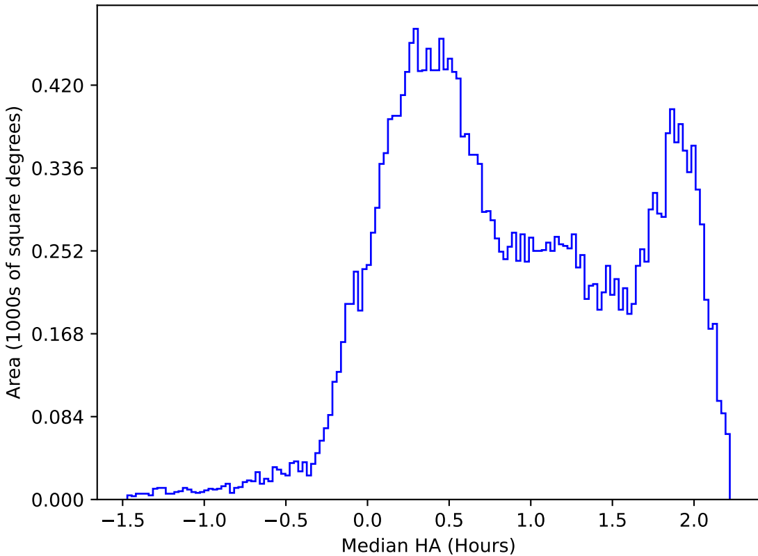
mw_roll_bulge_v3.3_10yrs All sky all bands: Median HA
