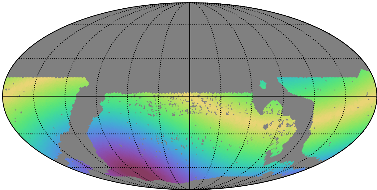
mw_roll_bulge_v3.3_10yrs WFD z band: Max solarElong
