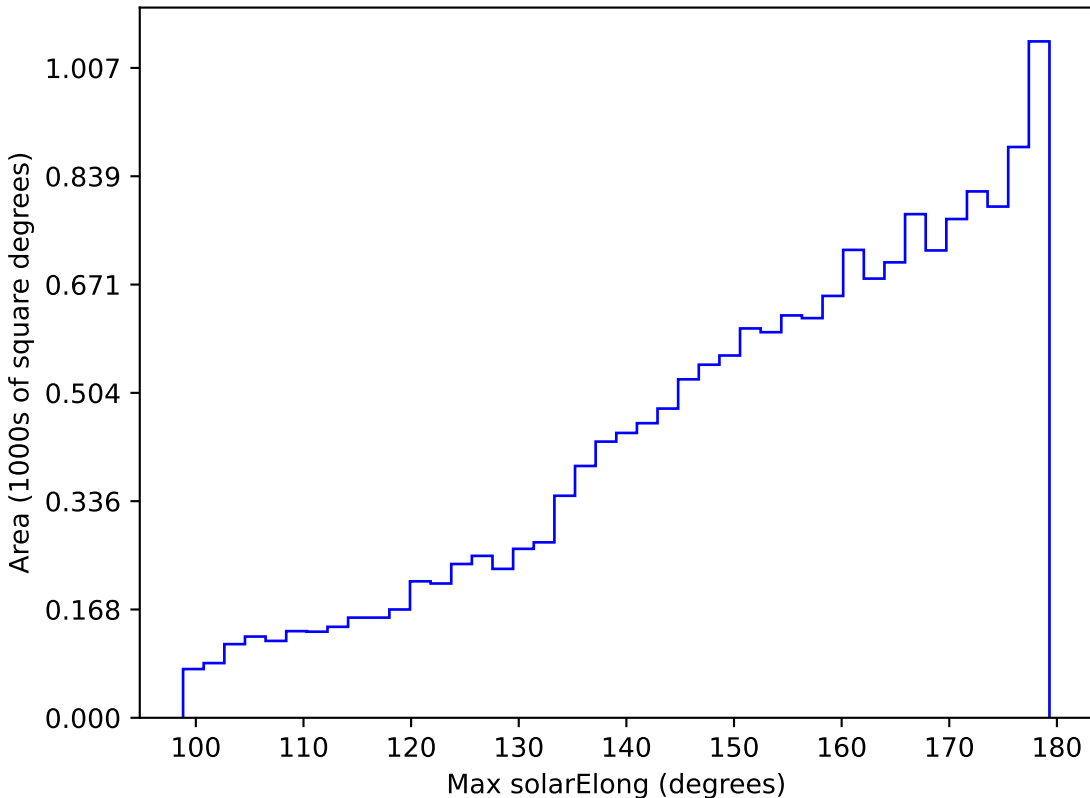
mw_roll_bulge_v3.3_10yrs WFD z band: Max solarElong
