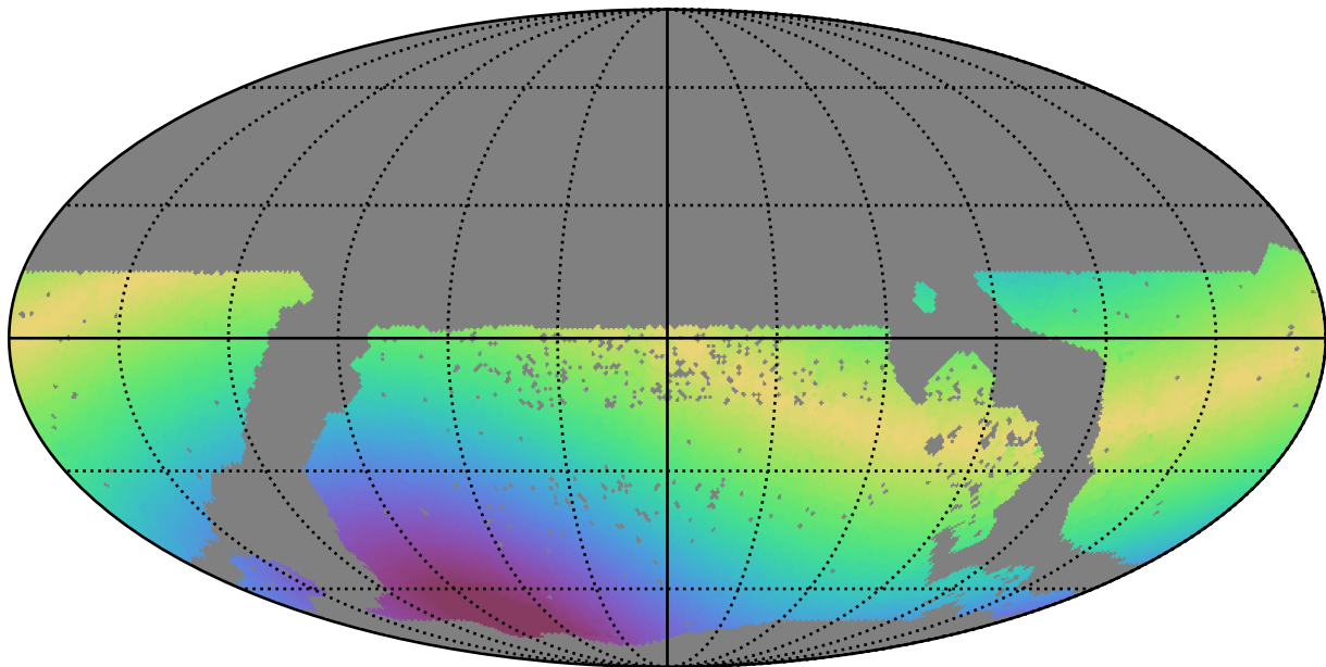
mw_roll_bulge_v3.3_10yrs WFD u band: Max solarElong
