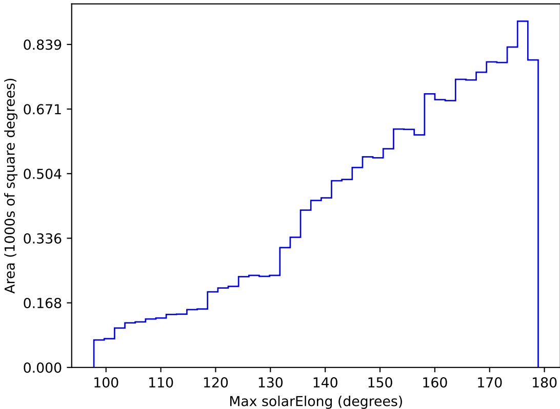
mw_roll_bulge_v3.3_10yrs WFD u band: Max solarElong
