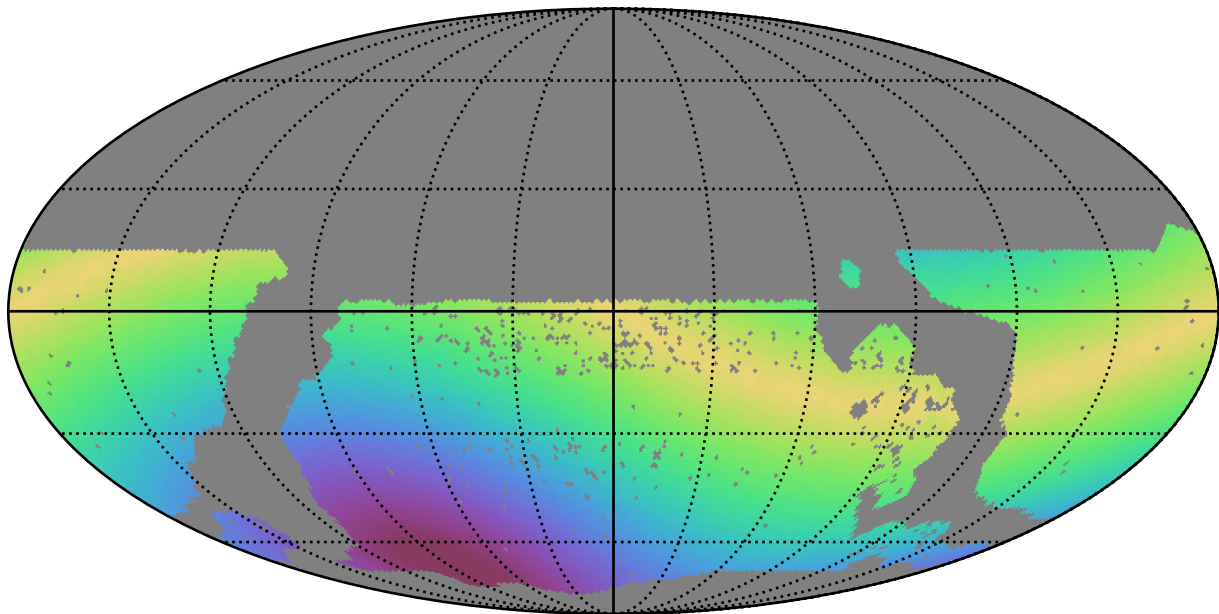
mw_roll_bulge_v3.3_10yrs WFD i band: Max solarElong
