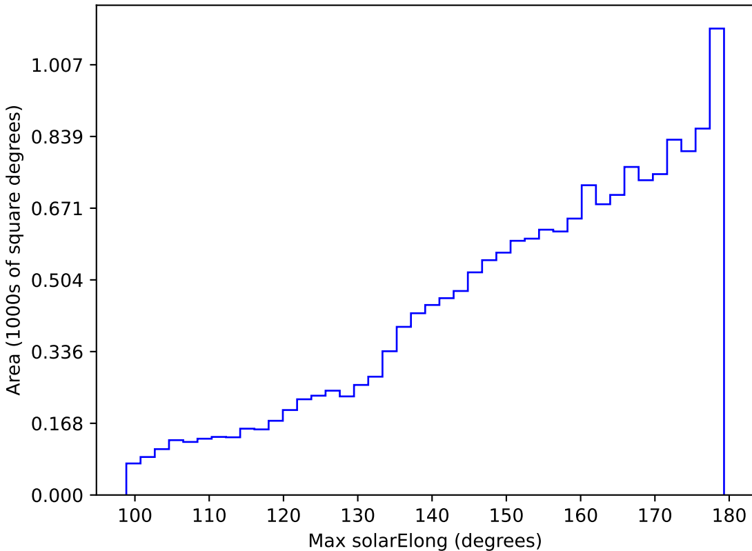
mw_roll_bulge_v3.3_10yrs WFD i band: Max solarElong
