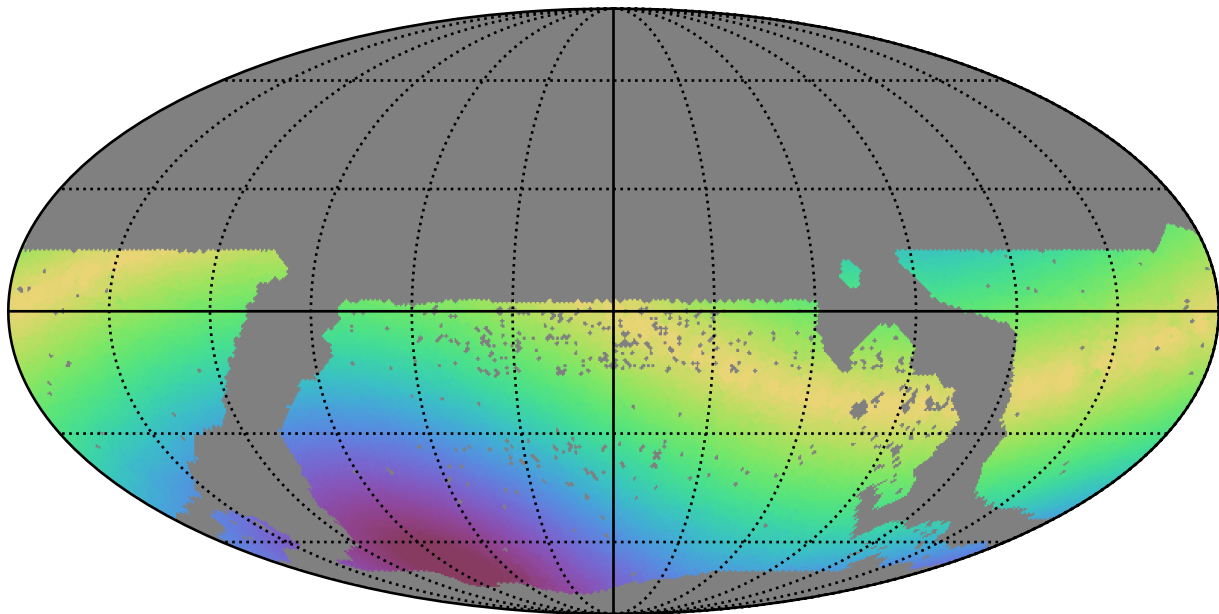
mw_roll_bulge_v3.3_10yrs WFD g band: Max solarElong
