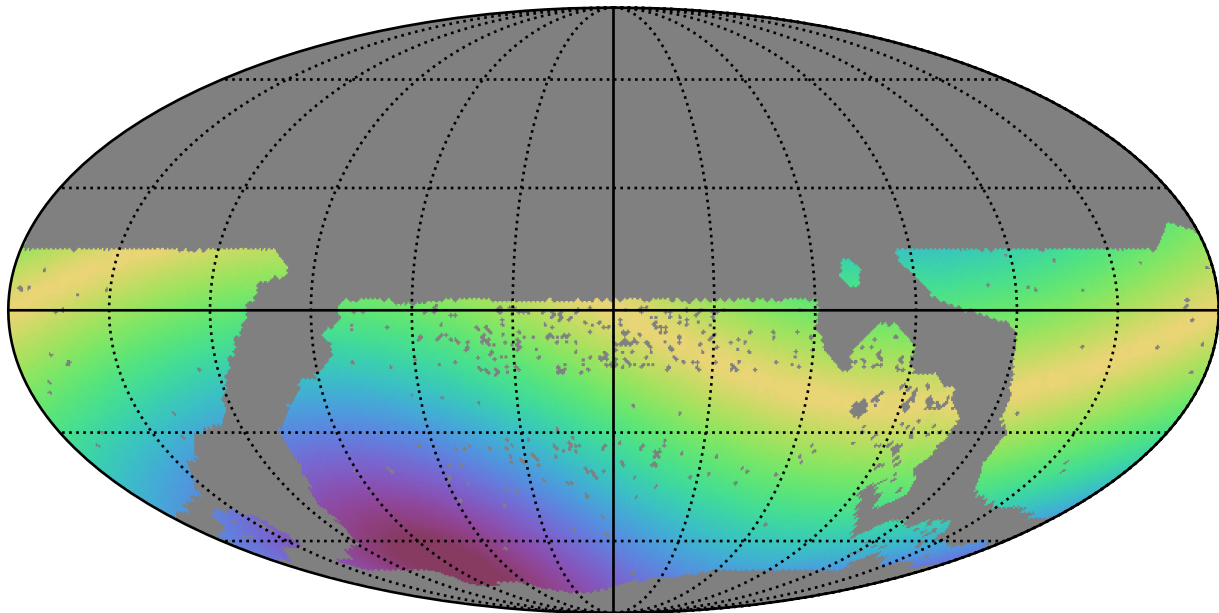
mw_roll_bulge_v3.3_10yrs WFD all bands: Max solarElong
