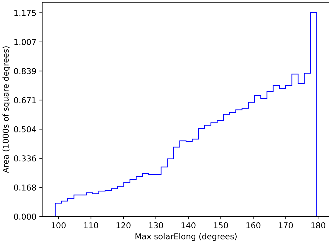
mw_roll_bulge_v3.3_10yrs WFD all bands: Max solarElong
