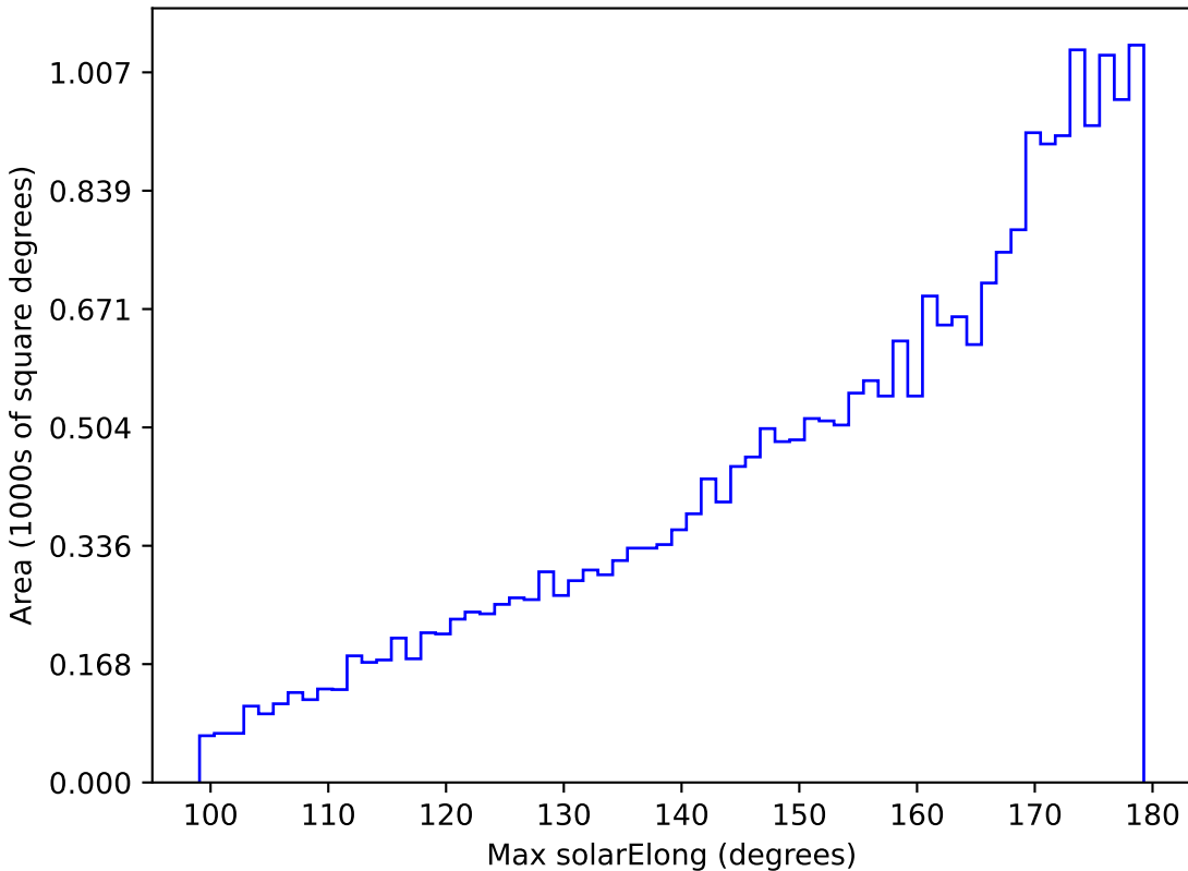
mw_roll_bulge_v3.3_10yrs All sky z band: Max solarElong
