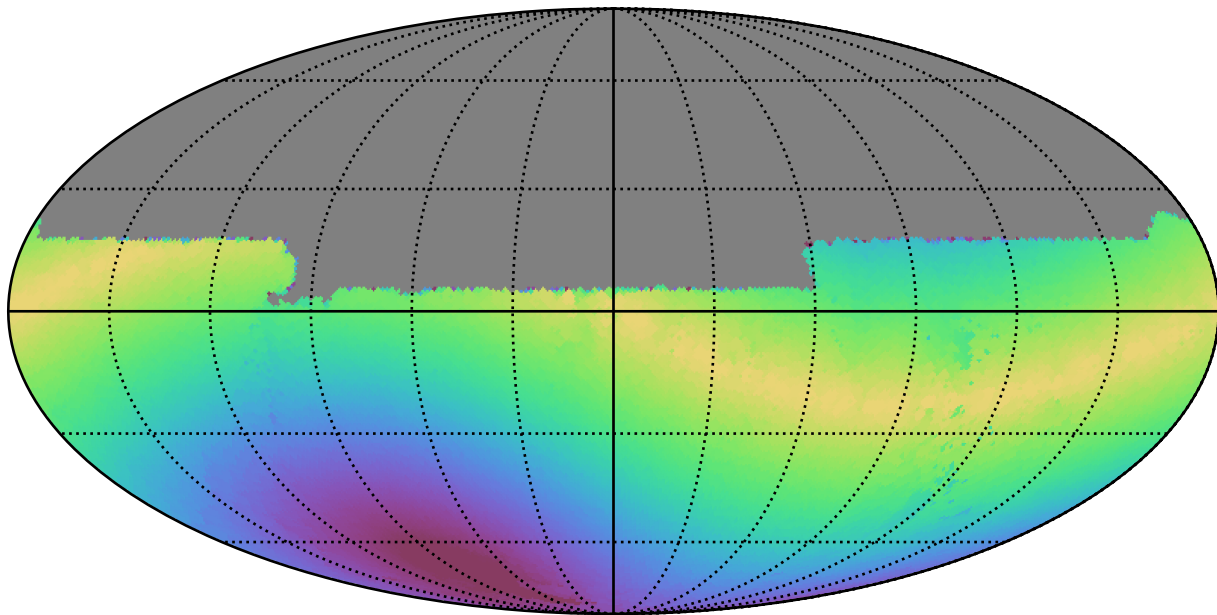
mw_roll_bulge_v3.3_10yrs All sky u band: Max solarElong
