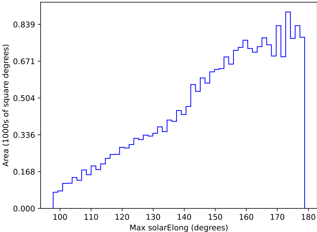
mw_roll_bulge_v3.3_10yrs All sky u band: Max solarElong
