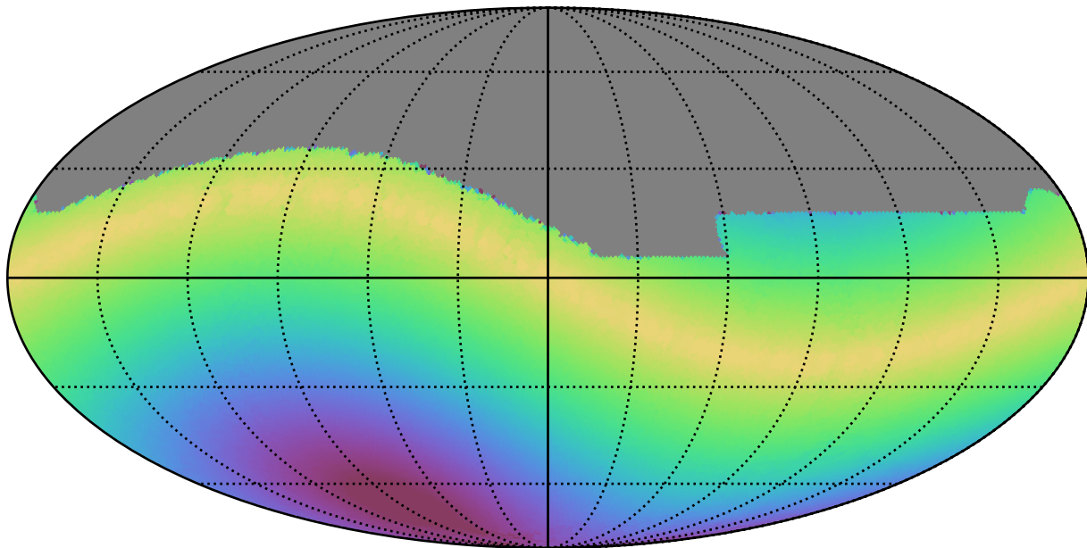
mw_roll_bulge_v3.3_10yrs All sky r band: Max solarElong
