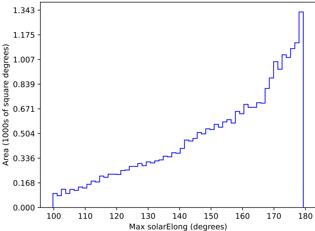
mw_roll_bulge_v3.3_10yrs All sky i band: Max solarElong
