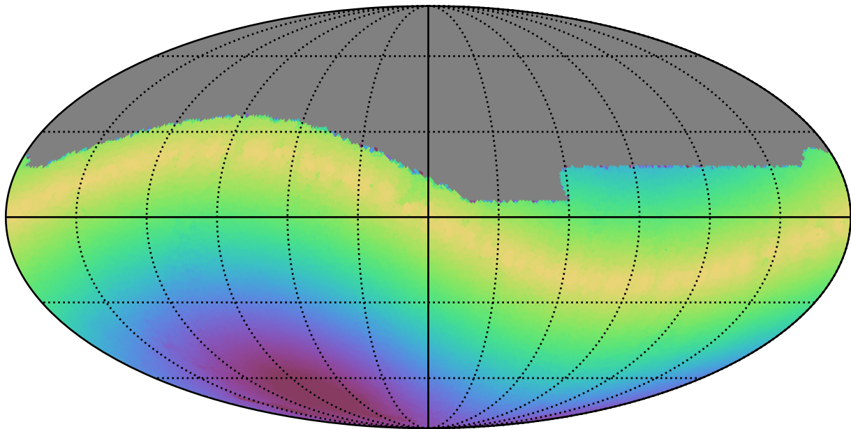
mw_roll_bulge_v3.3_10yrs All sky g band: Max solarElong
