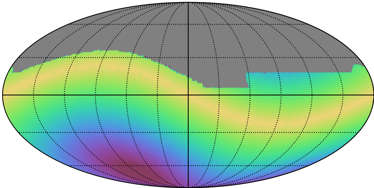
mw_roll_bulge_v3.3_10yrs All sky all bands: Max solarElong
