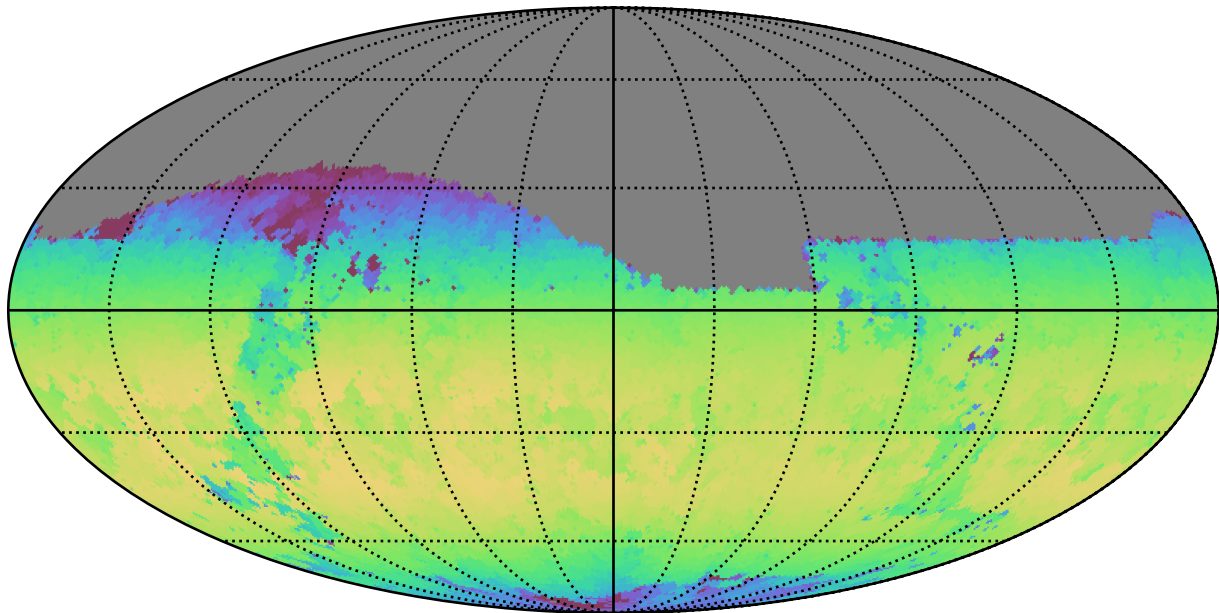
mw_roll_bulge_v3.3_10yrs Yr 1 z band: Max skyBrightness
