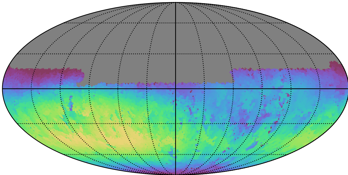
mw_roll_bulge_v3.3_10yrs Yr 1 u band: Max skyBrightness
