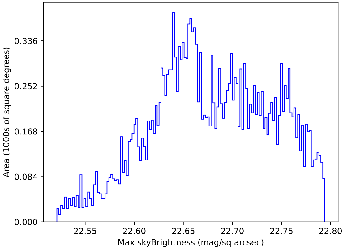
mw_roll_bulge_v3.3_10yrs Yr 1 u band: Max skyBrightness
