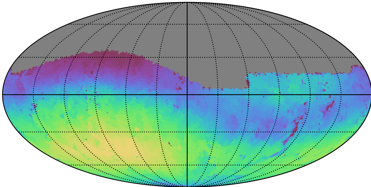
mw_roll_bulge_v3.3_10yrs Yr 1 g band: Max skyBrightness
