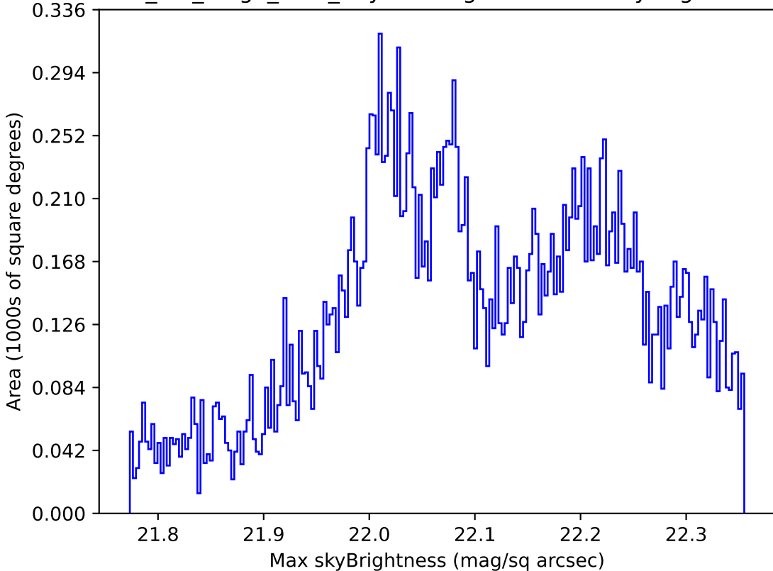
mw_roll_bulge_v3.3_10yrs Yr 1 g band: Max skyBrightness
