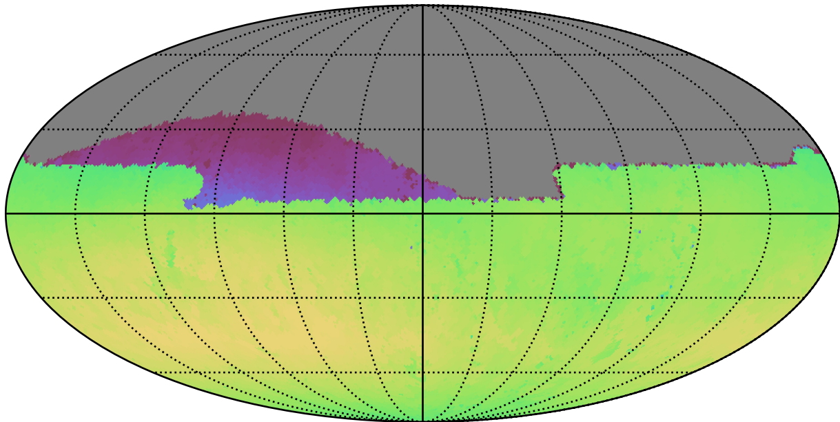
mw_roll_bulge_v3.3_10yrs Yr 1 all bands: Max skyBrightness
